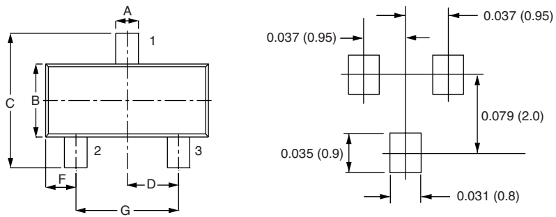
Soldering pad
